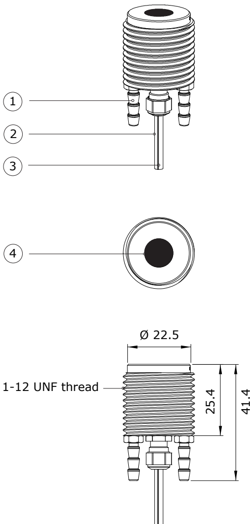
Figure 5 optional SBG01-T from top to bottom: 3D view, front view, side view. Dimensions in \times 10^{-3} m. (1) water cooling tube, outer diameter tubes 4.2 \times 10^{-3} m, (2) cable, (3) thermocouple cable, standard cable length is 2 m, (4) thermopile sensor with black coating
